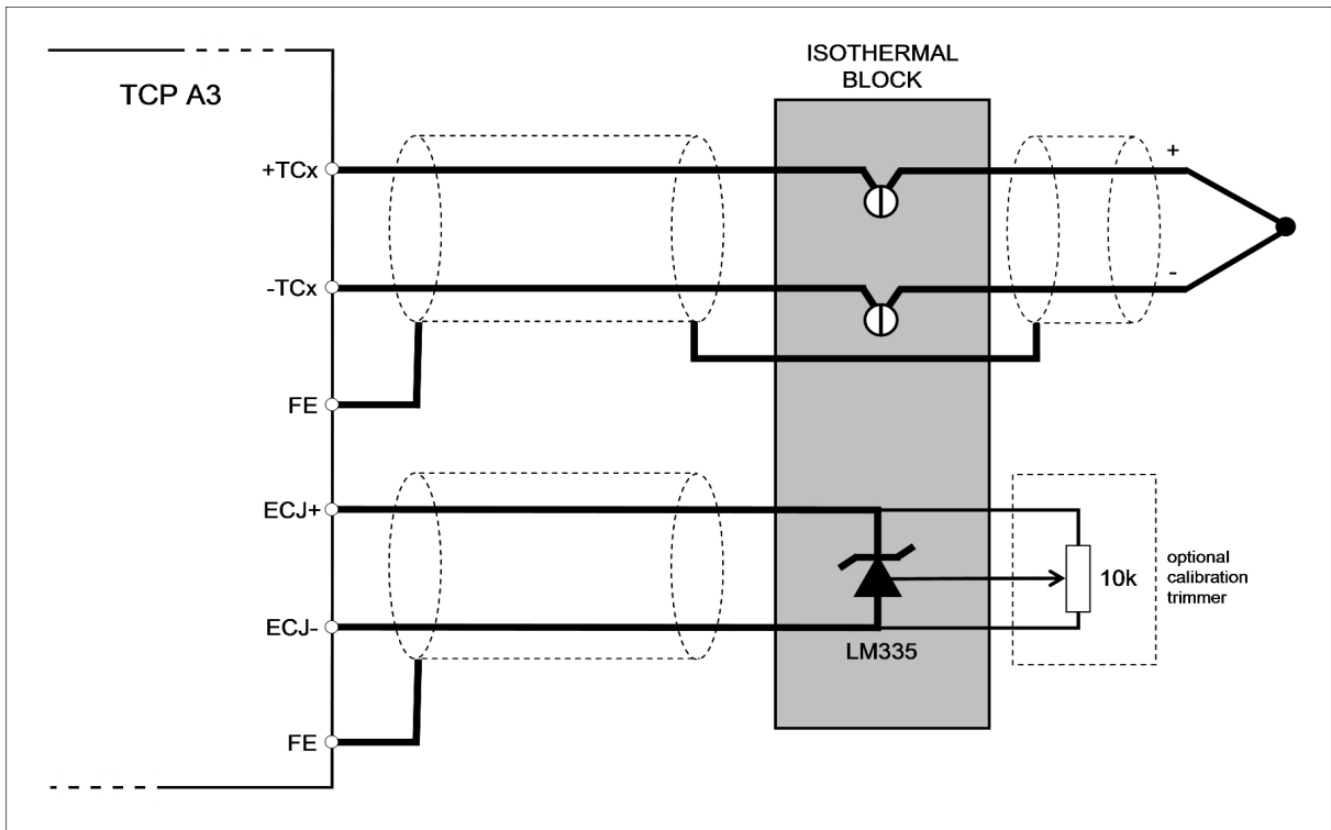
Recommended connections for thermocouples, using external cold junction sensor and junction box.
