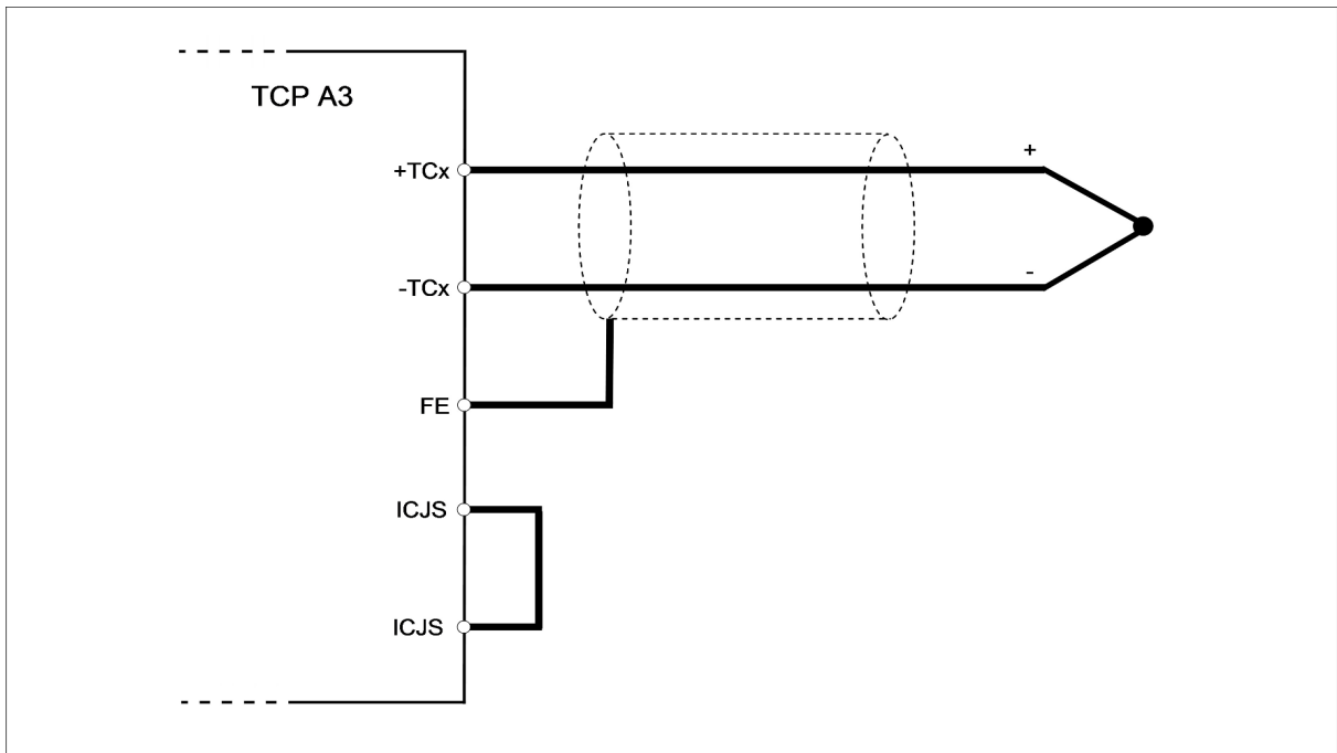
Recommended connections for thermocouples, using internal cold junction sensor.
