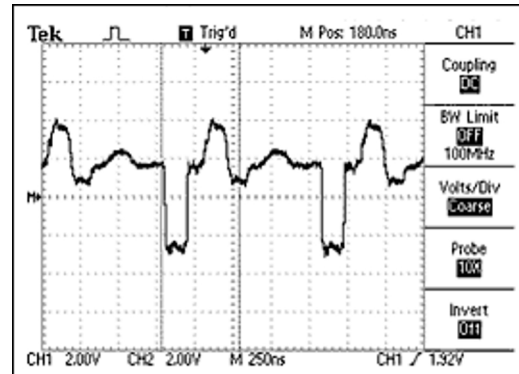
Example of a signal with incorrect value terminations
