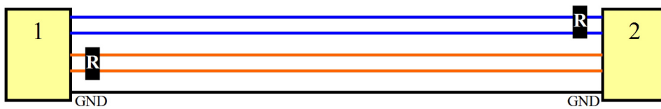
Example of RS422 wiring
